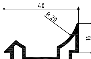
420190 ESQUINERO REGULABLE
