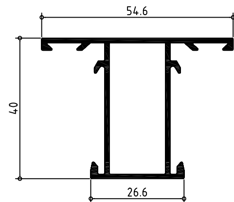
420705 PILASTRA 40 X 20
