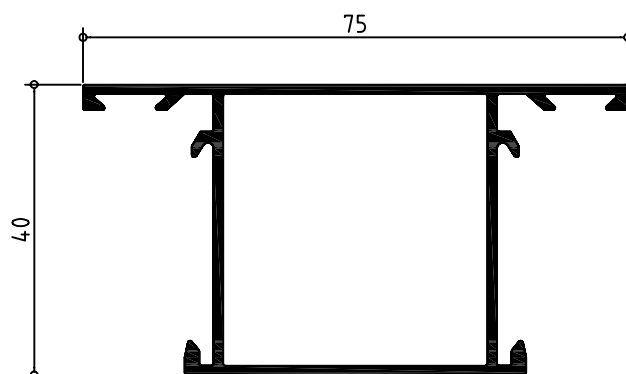
440705 PILASTRA 40 X 40
