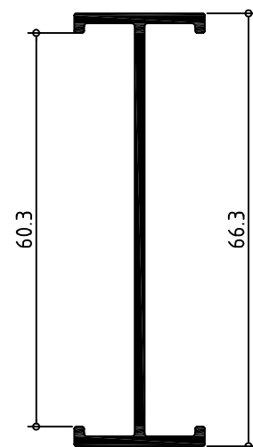
072860 UNION MARCO LATERALES
