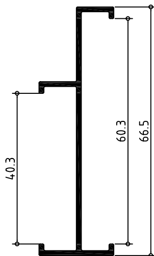
072750 UNION CORREDERA ABATIBLE
