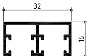
065225 GUIA SUPERIOR
